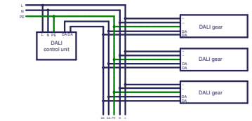
Sample DALI wiring diagram:
