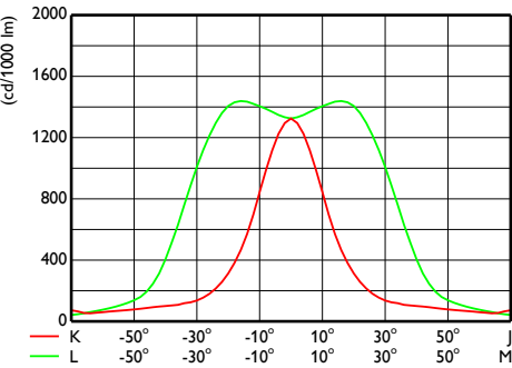
OFCS1_BVP1301xLED260-4S740S
