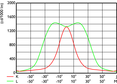
OFCS1_BVP130T251xLED260-4S740S
