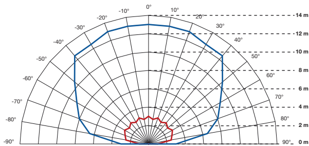
Reikwijdte IS 2180-2, 12 m lens (blauw = tangenciale loopricting, rood = radiale loopricting)
