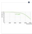
CDM-TC 20W /830 on electronic gear + Zoom
